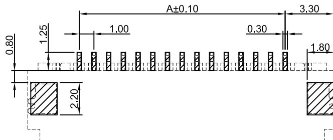
P.C.B LAYOUT (TOP VIEW) TOLERANCE:±0.05
