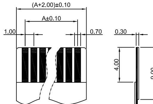
APPLICABLE FFC/FPC TOLERANCE:±0.05
