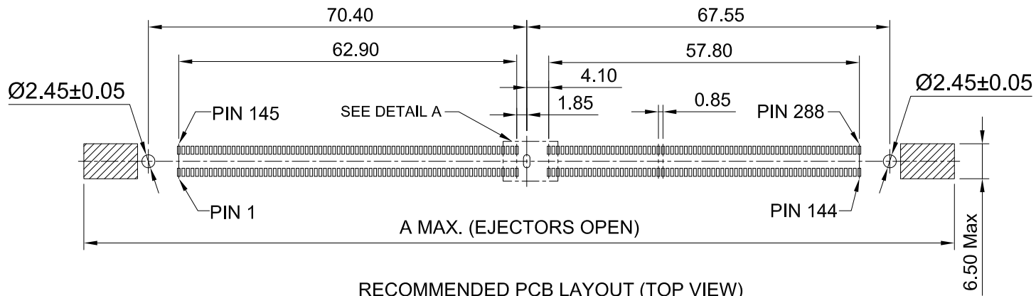
RECOMMENDED PCB LAYOUT (TOP VIEW) TYPE F1 BOARDLOCKS
