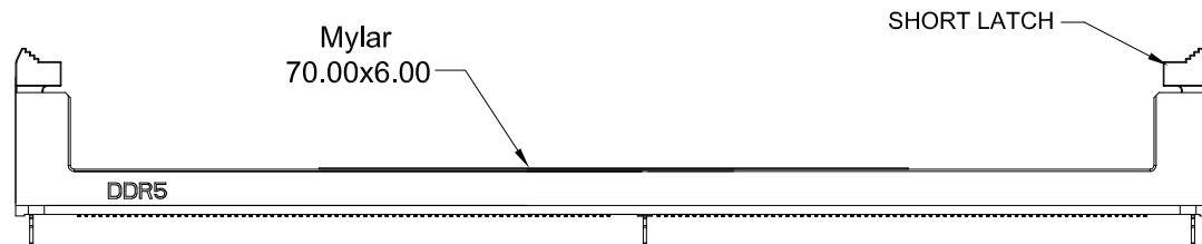
SHORT LATCH
