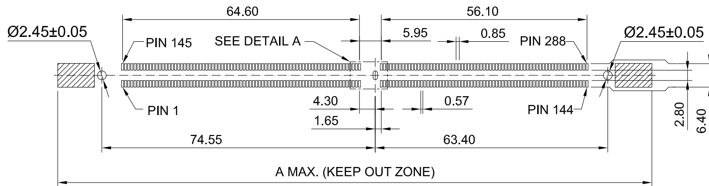
RECOMMENDED PCB LAYOUT (TOP VIEW) TYPE F1 BOARDLOCKS
