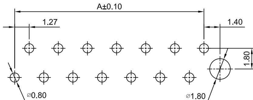
P.C.B LAYOUT TOLERANCE:±0.05
