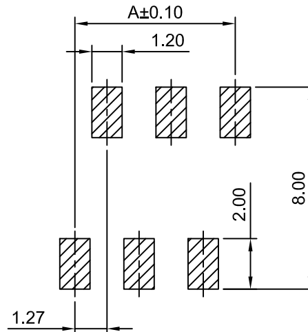
P.C.B LAYOUT TOLERANCE:±0.05
