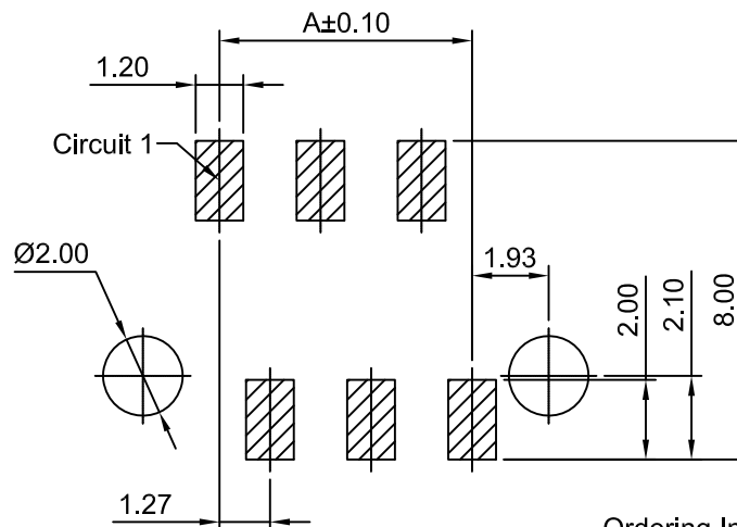
P.C.B LAYOUT TOLERANCE:±0.05
