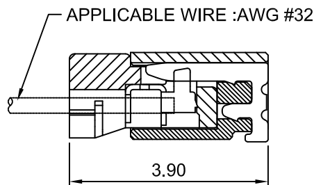
MATED CONDITION
