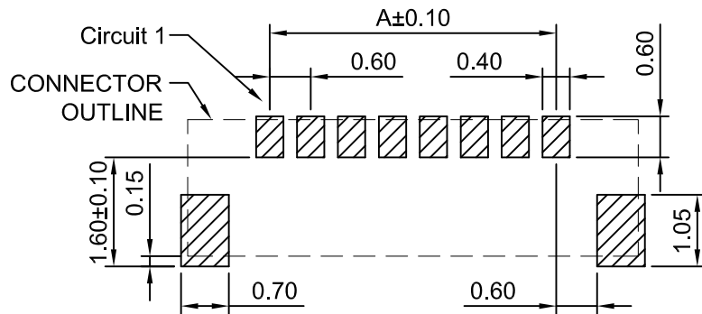
P.C.B LAYOUT (TOP VIEW) TOLERANCE: ±0.05
