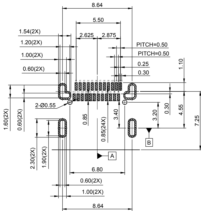
RECOMMENDED PCB LAYOUT(TOP VIEW) THICKNESS 0.60MM;DEFAULT TOLERANCE:±0.05
