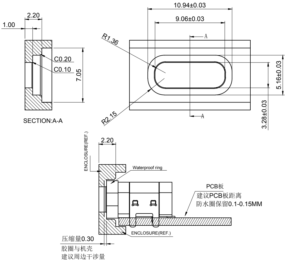
RECOMMENDED SCHEMATIC DRAWING OF CONNECTOR MATCH CHASSIS
