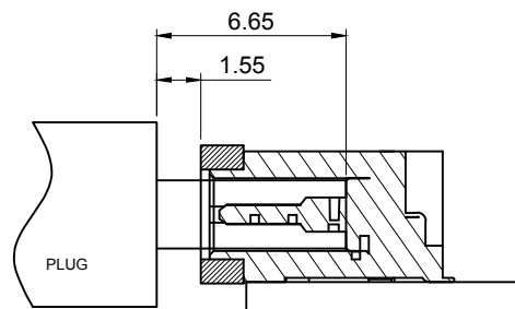
MATED CONDITION(REF.)
