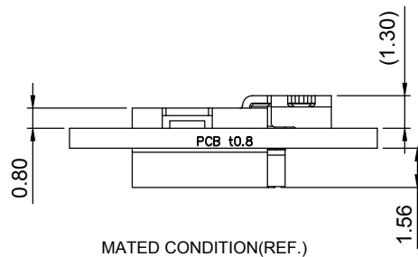
MATED CONDITION(REF.)
