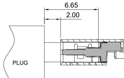
MATED CONDITION(REF.)
