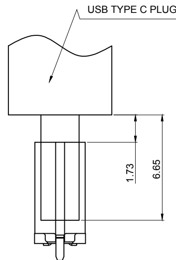
FEMALE AND MALE MATCHING DRAWING
