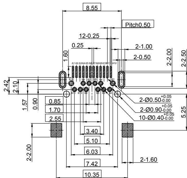
RECOMMENDED PCB LAYOUT(TOP VIEW) PCB THICKNESS 1.2±0.05MM
