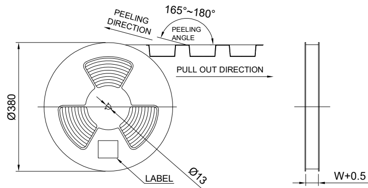
REEL VIEW
