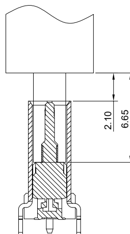
Mated Condition(Ref.)
