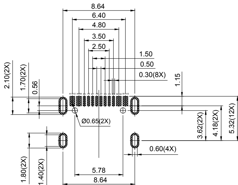
RECOMMENDED PCB LAYOUT(TOP VIEW) THICKNESS 0.80MM;DEFAULT TOLERANCE:±0.05
