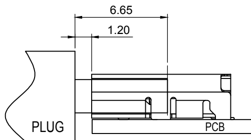
Mated Condition(REF.)
