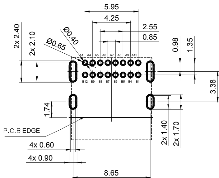
RECOMMENDED PCB LAYOUT(TOP) TOLERANCES:±0.05MM
