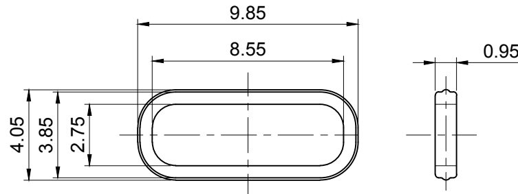
Waterproof Ring Size Chart
