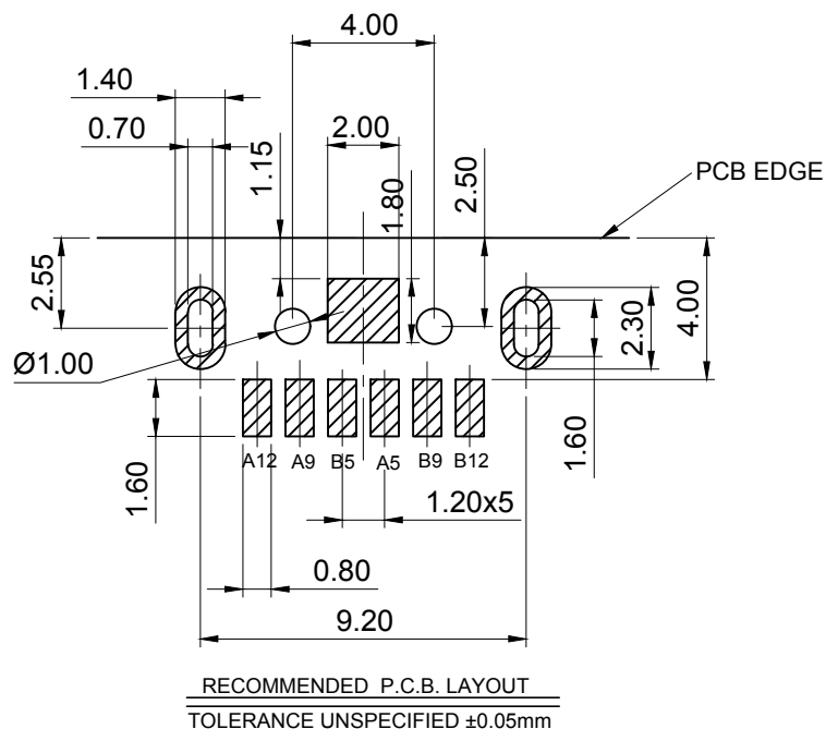
USB Type-C Pin Assignments
