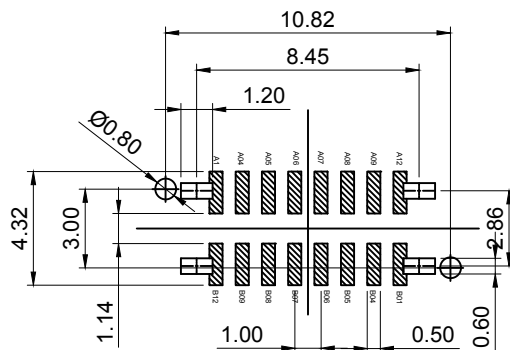
RECOMMENDED P.C.B. LAYOUT TOLERANCE UNSPECIFIED \pm 0.05\text{mm}
