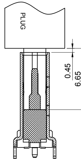
AFTER MATING
