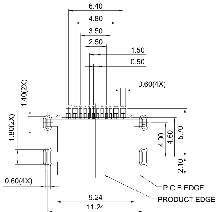
RECOMMENDED PCB LAYOUT(TOP VIEW) THICKNESS 0.80MM;DEFAULT TOLERANCE:±0.05
