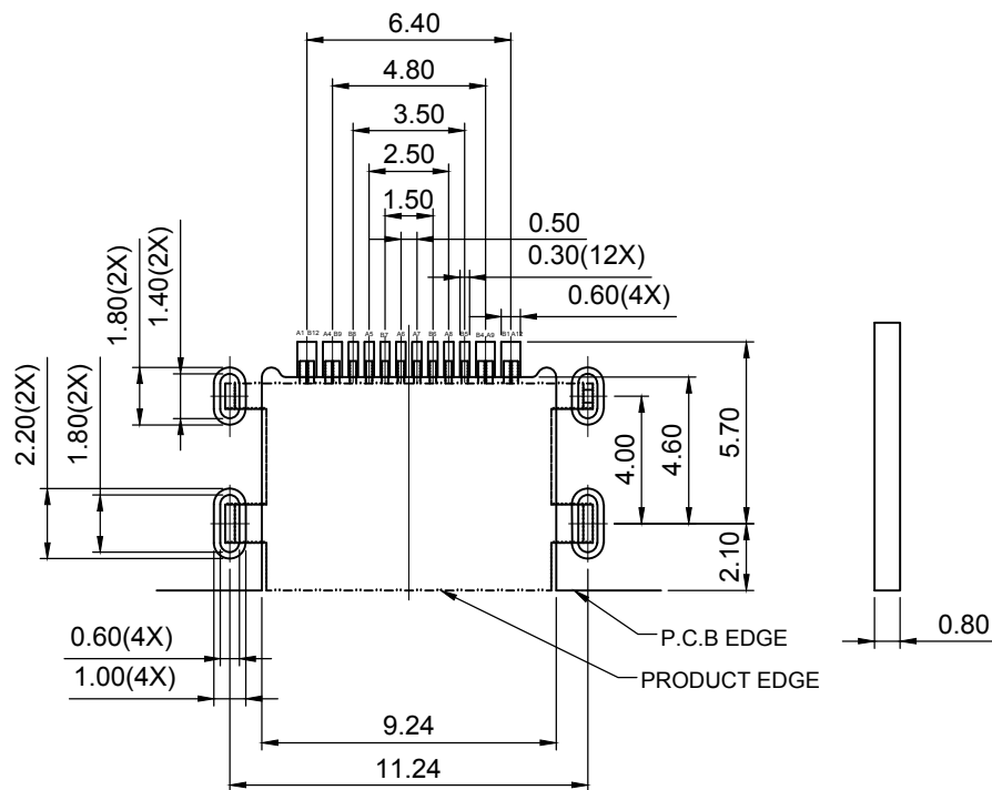
RECOMMENDED PCB LAYOUT(TOP VIEW) THICKNESS 0.80MM;DEFAULT TOLERANCE:±0.05
