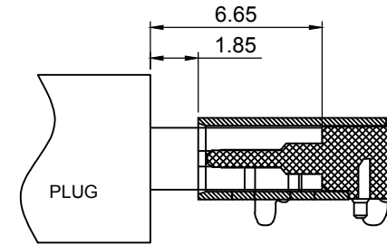
Mated Condition(REF.)
