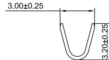
SEC B-B
