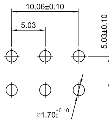
P.C.B LAYOUT TOLERANCE:±0.05
