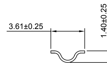
SEC:C-C
