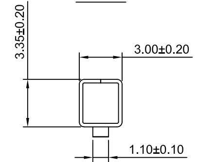
SEC:C-C
