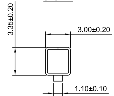
SEC:C-C
