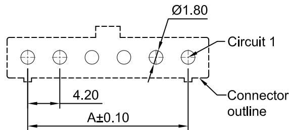
P.C.B LAYOUT (TOP VIEW) TOLERANCE: ±0.05
