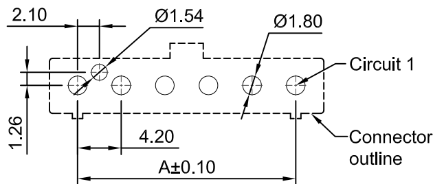
P.C.B LAYOUT(TOP VIEW) TOLERANCE:±0.05
