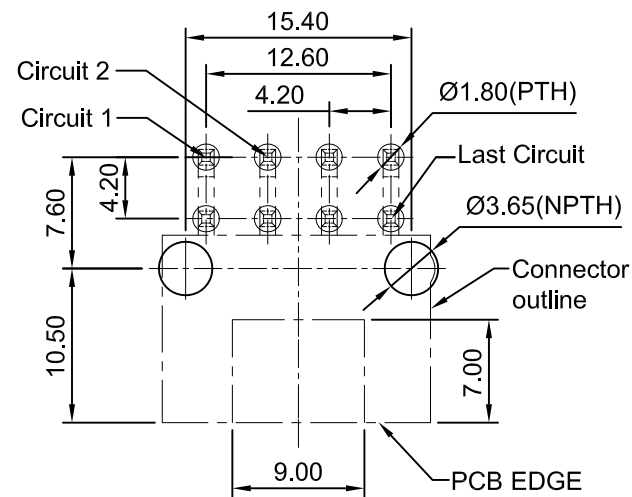
RECOMMEND P.C.B LAYOUT(PIP) TOLERANCE \pm 0.05 TOP VIEW
