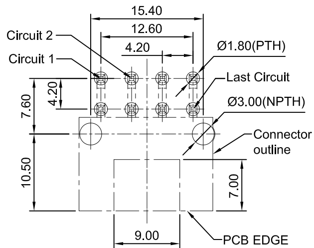
RECOMMEND P.C.B LAYOUT(DIP) TOLERANCE \pm 0.05 TOP VIEW
