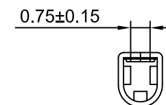
SEC:C-C
