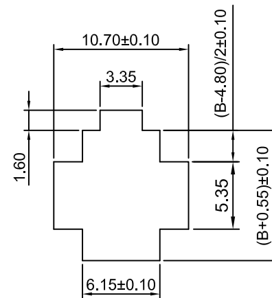
Panel hole layout (2P~3P)
