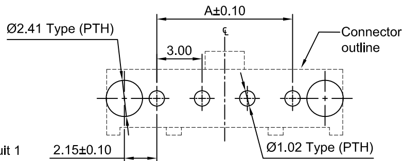
P.C.B LAYOUT TOLERANCE:±0.05
