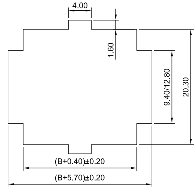
Panel Hole Layout
