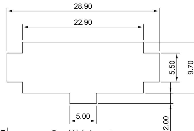
Panel Hole Layout Thickness:1.00~1.80
