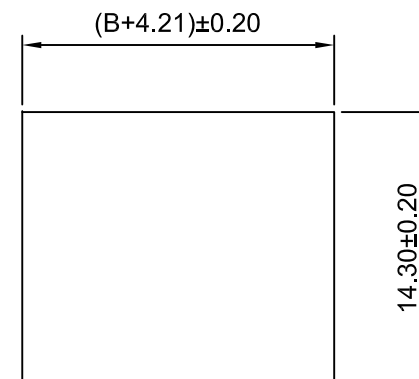
Panel hole layout
