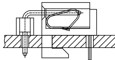
Mating Draw
