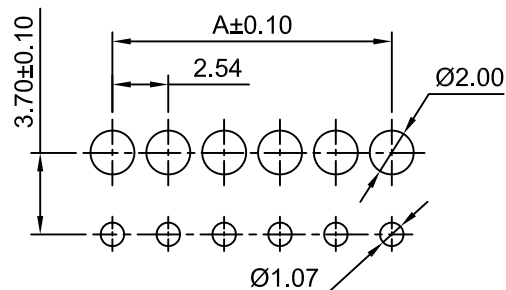
P.C.B LAYOUT TOLERANCE:±0.05
