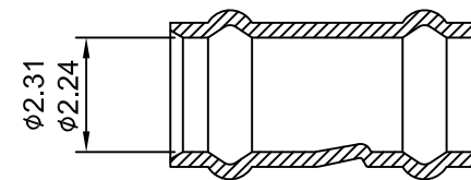
SEC:C-C
