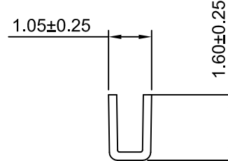
SEC:C-C
