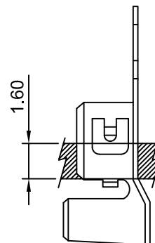
Assembly Layout
