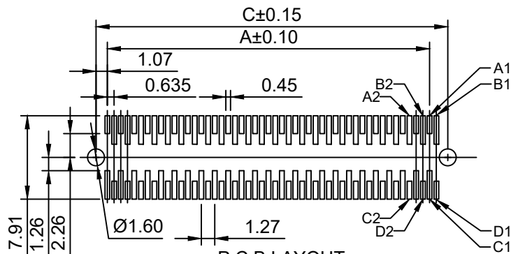
P.C.B LAYOUT TOLERANCE:±0.05
