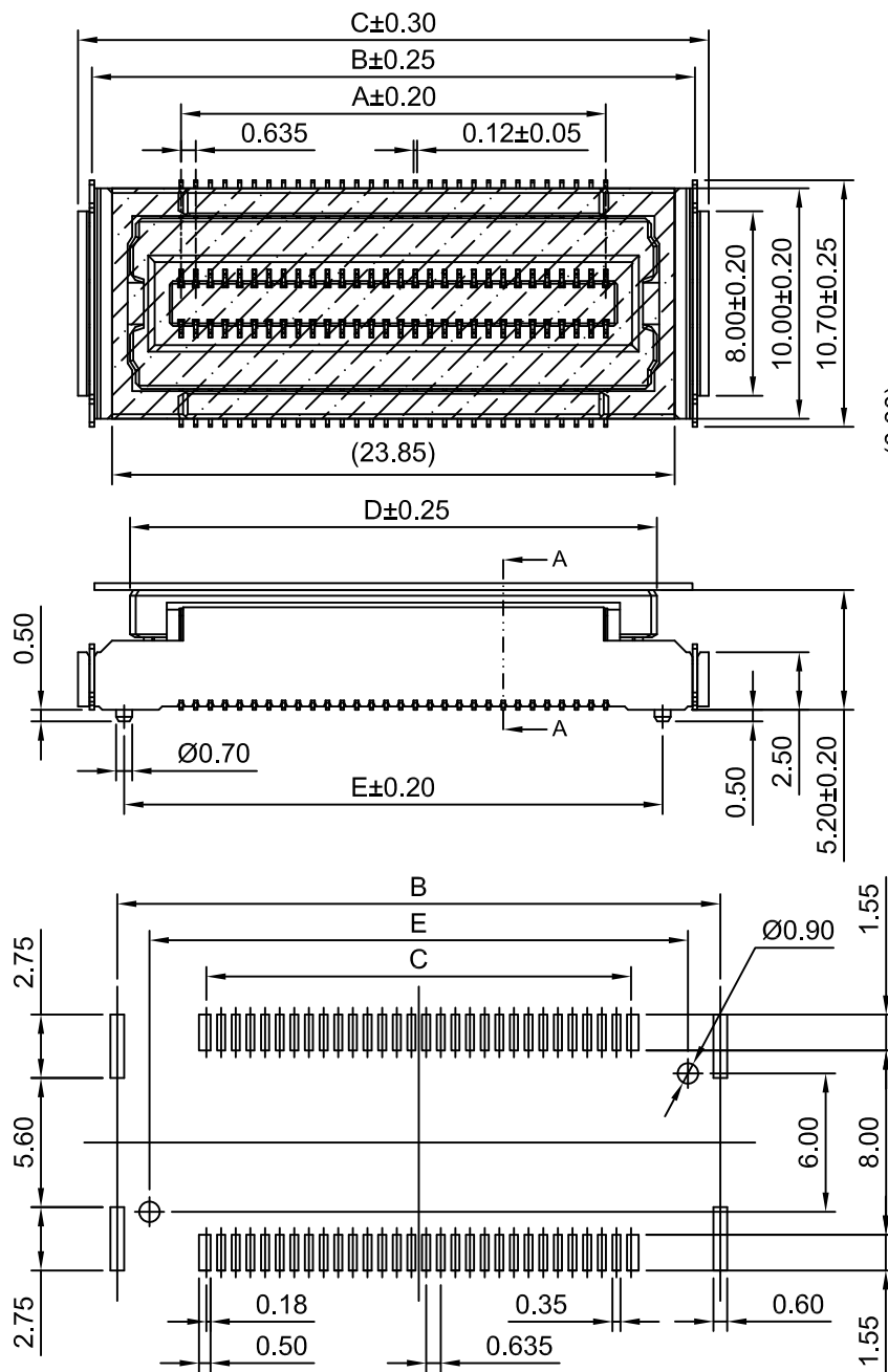
P.C.B LAYOUT TOLERANCE: \pm 0.05
