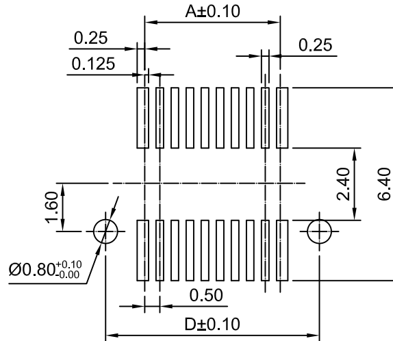
P.C.B LAYOUT TOLERANCE:±0.05
