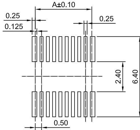
P.C.B LAYOUT TOLERANCE:±0.05
