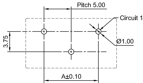
Component Side [A7921WVI-XP-**-2-A]
