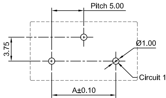
Component Side [A7921WVI-XP-**-A]
