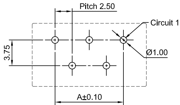
Odd Numbers Component Side [A7921WVI-XP-**-2]
