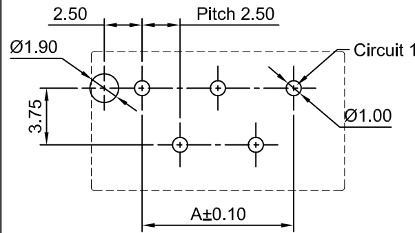
Odd Numbers Component Side [A7921WVI-F-XP-**-2]
