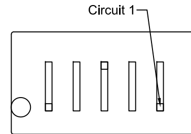
Solder Side [A7921WVI-F-XP-**-2-A]
