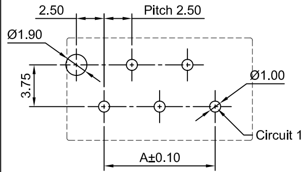
Odd Numbers Component Side [A7921WVI-F-XP-**]
