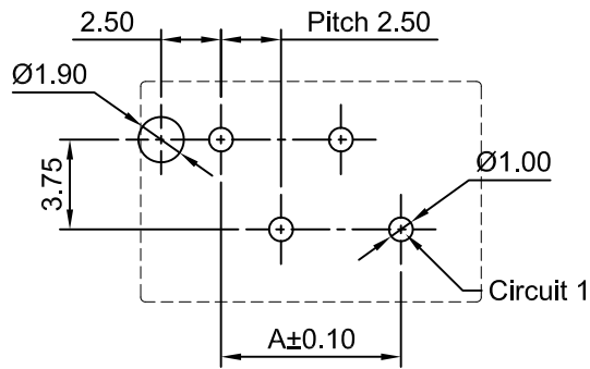
Even Numbers Component Side [A7921WVI-F-XP-**-2]
