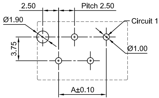
Even Numbers Component Side [A7921WVI-F-XP-**]
