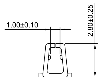
SEC:C-C
